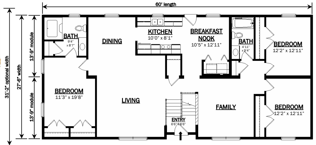
The CULPMONT 27'6" x 60 Raised Ranch *31'2" optional width 1650 SqFt 3 BR
