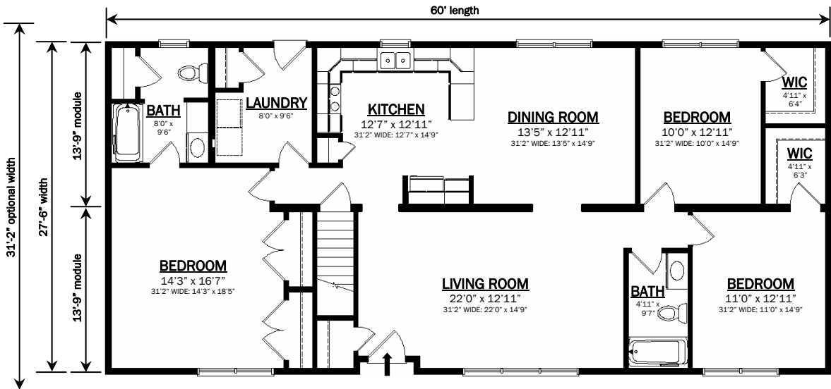
The MILLER 27'6" x 60 Ranch *31'2" optional width
