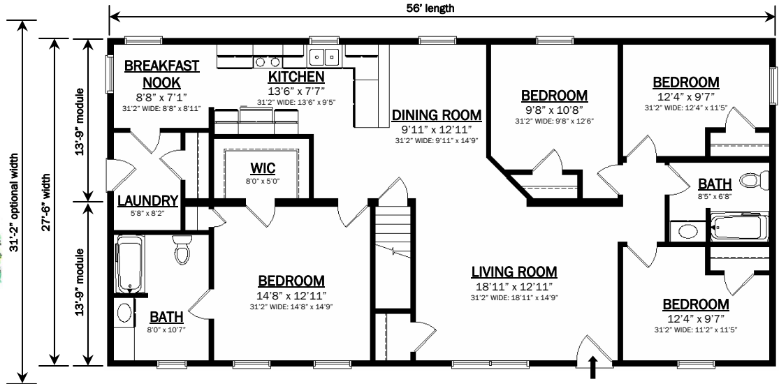
The TRAFALGER 27'6" x 56 Ranch *31'2" optional width 1540 SqFt 4 BR
