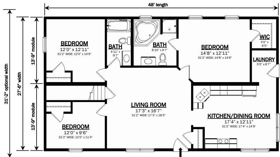
The MORNING GLORY 27'6" x 48 Ranch *31'2" optional width 1320 SqFt 3BR
