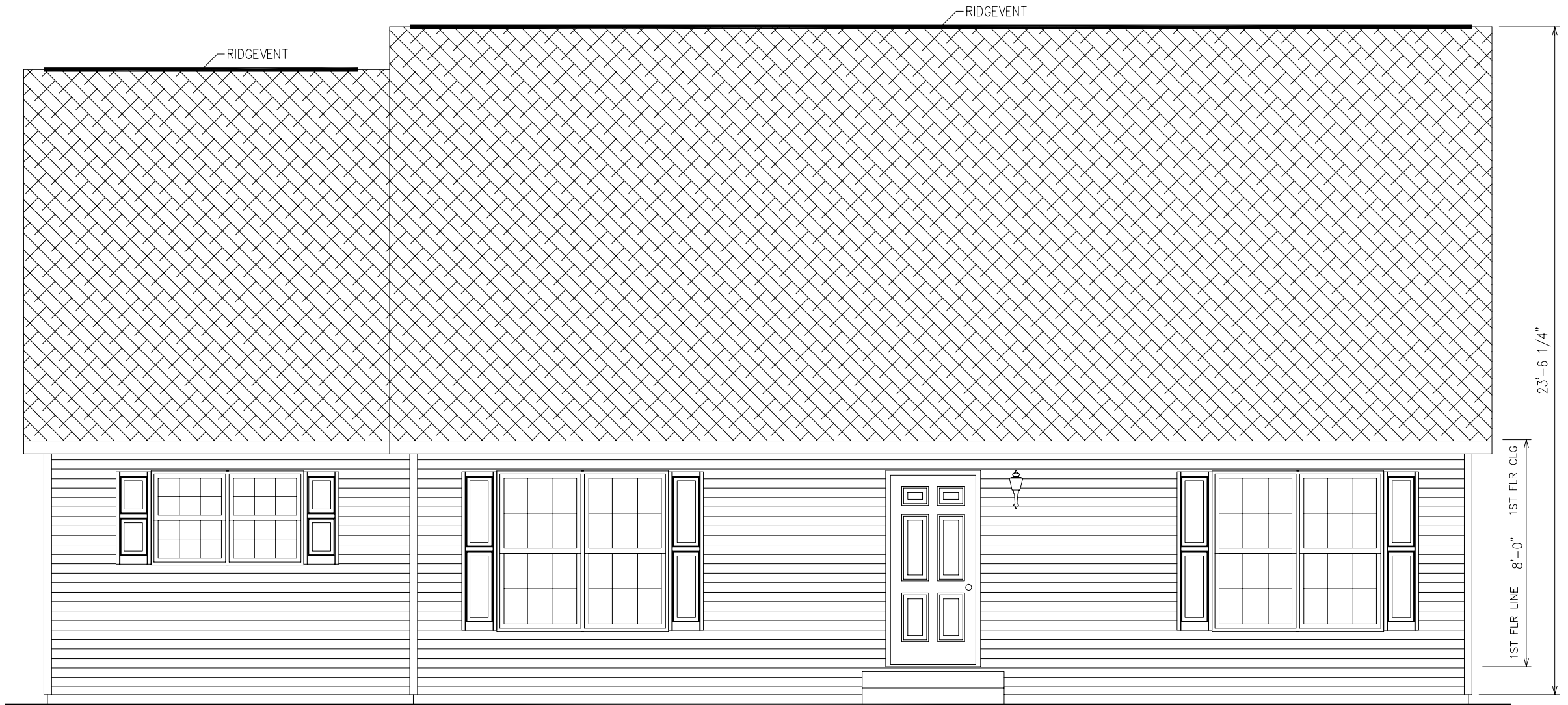
FRONT ELEVATION
