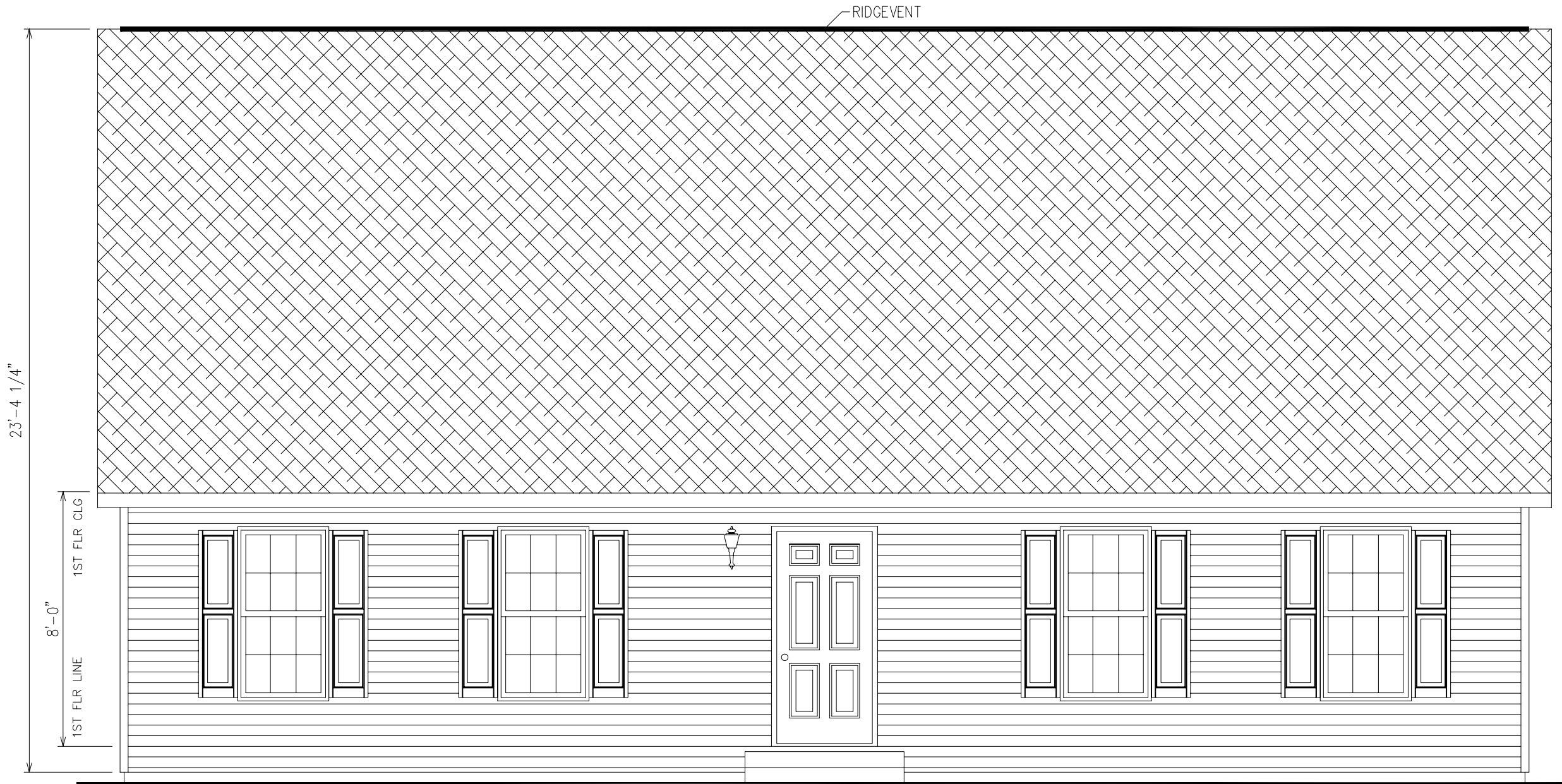
FRONT ELEVATION
