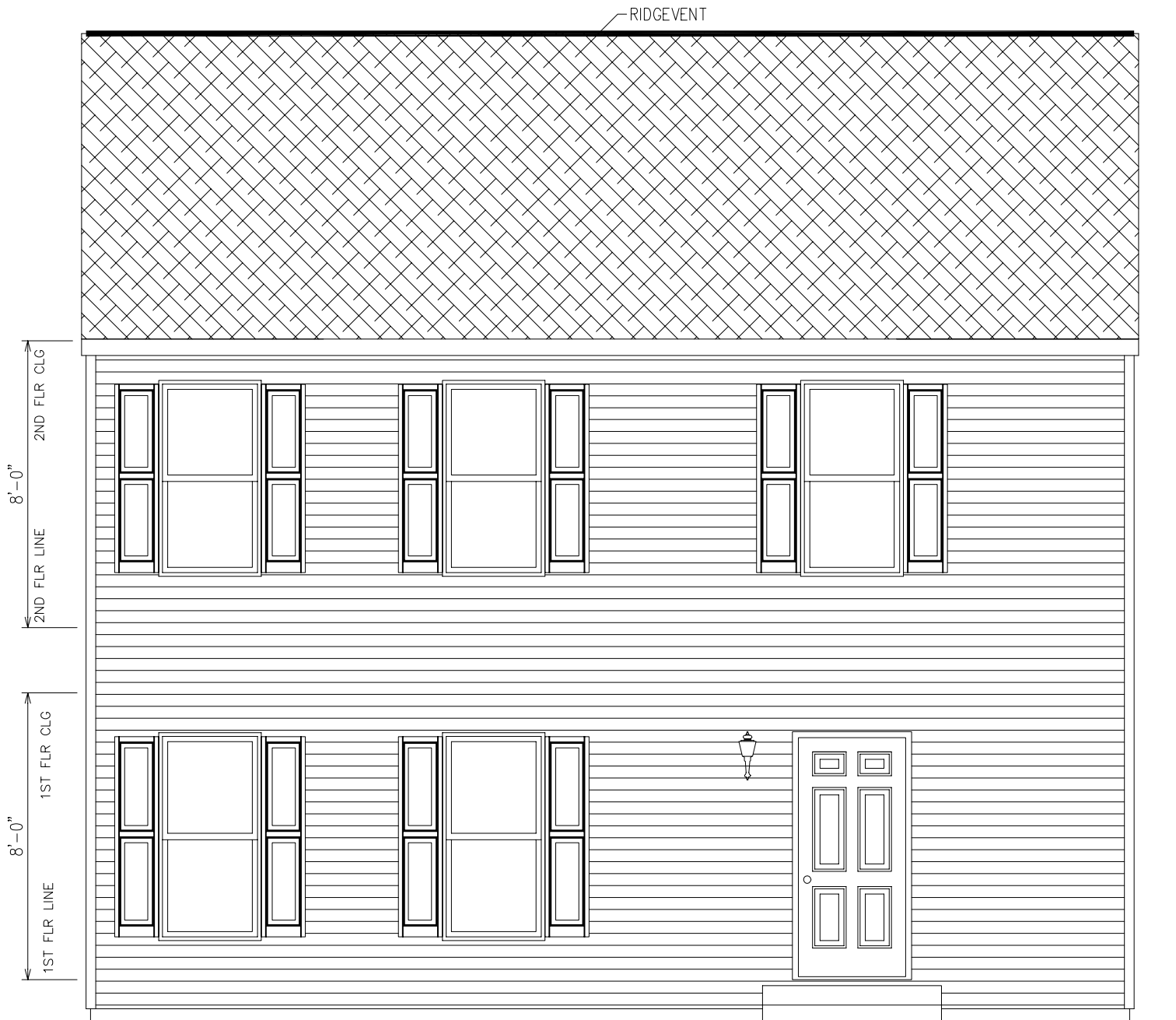
FRONT ELEVATION
