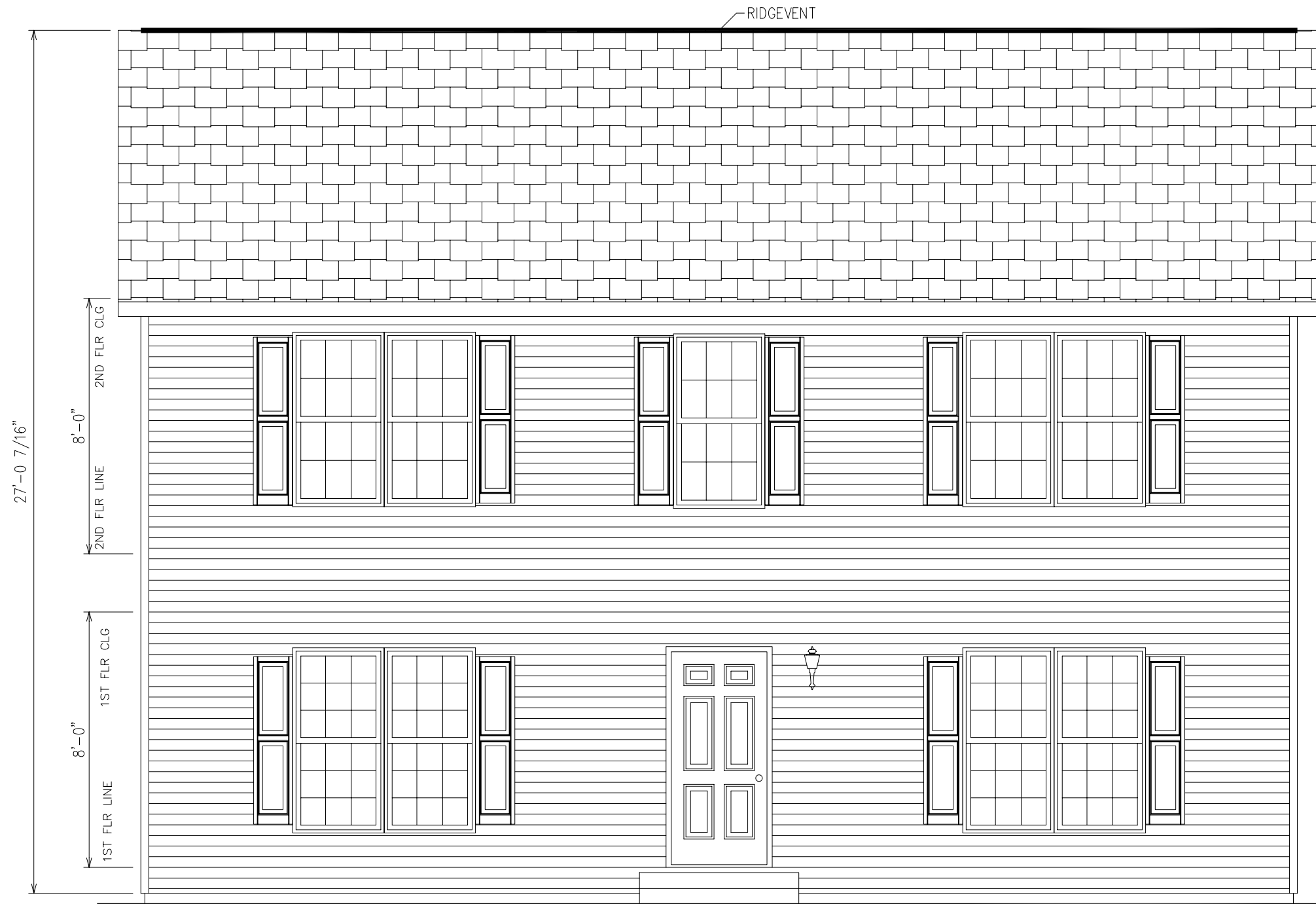
FRONT ELEVATION
