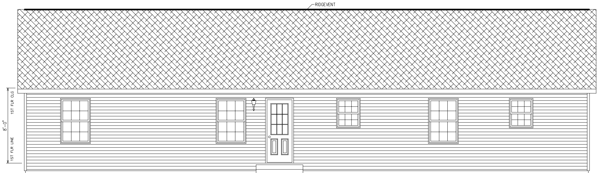
FRONT ELEVATION
