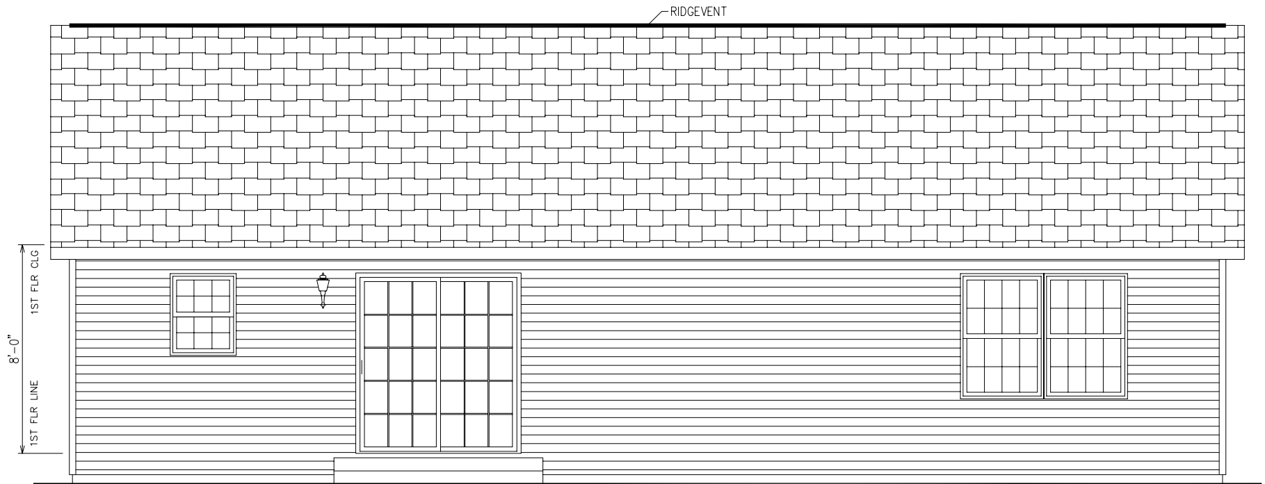
REAR ELEVATION
