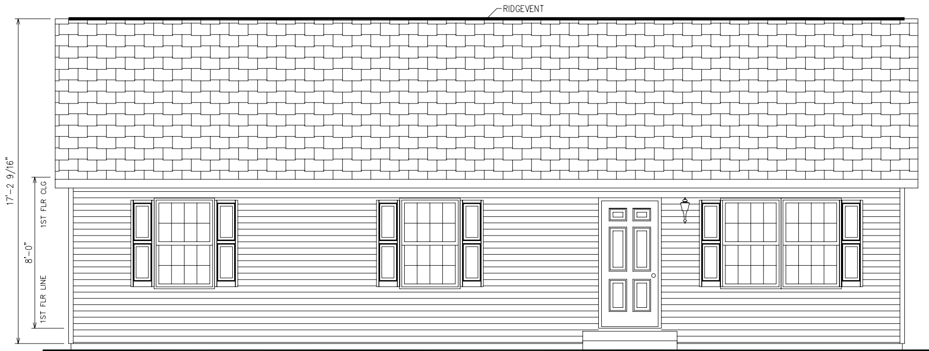
FRONT ELEVATION
