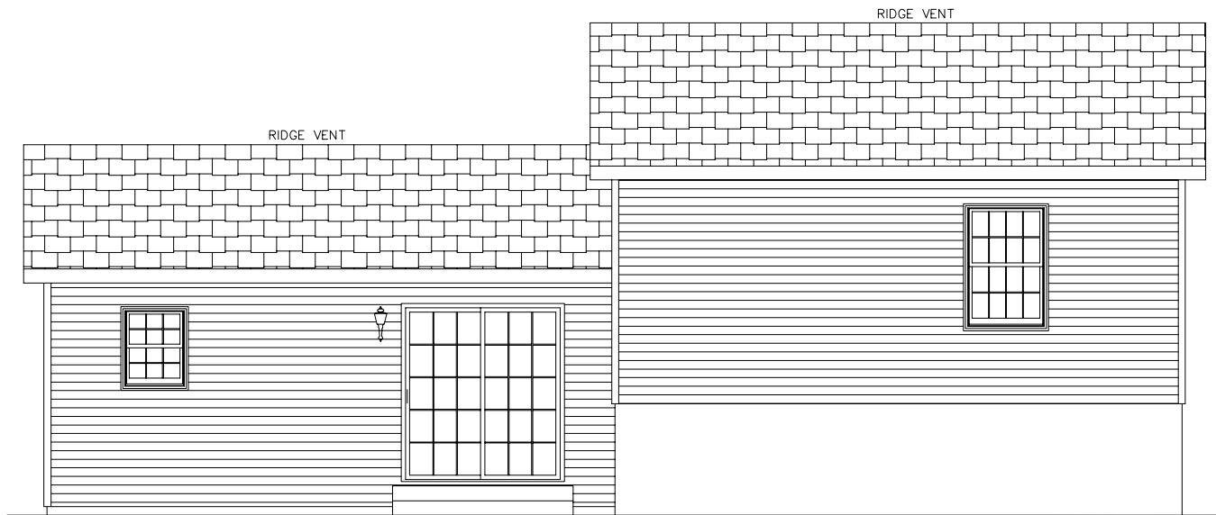
REAR ELEVATION
