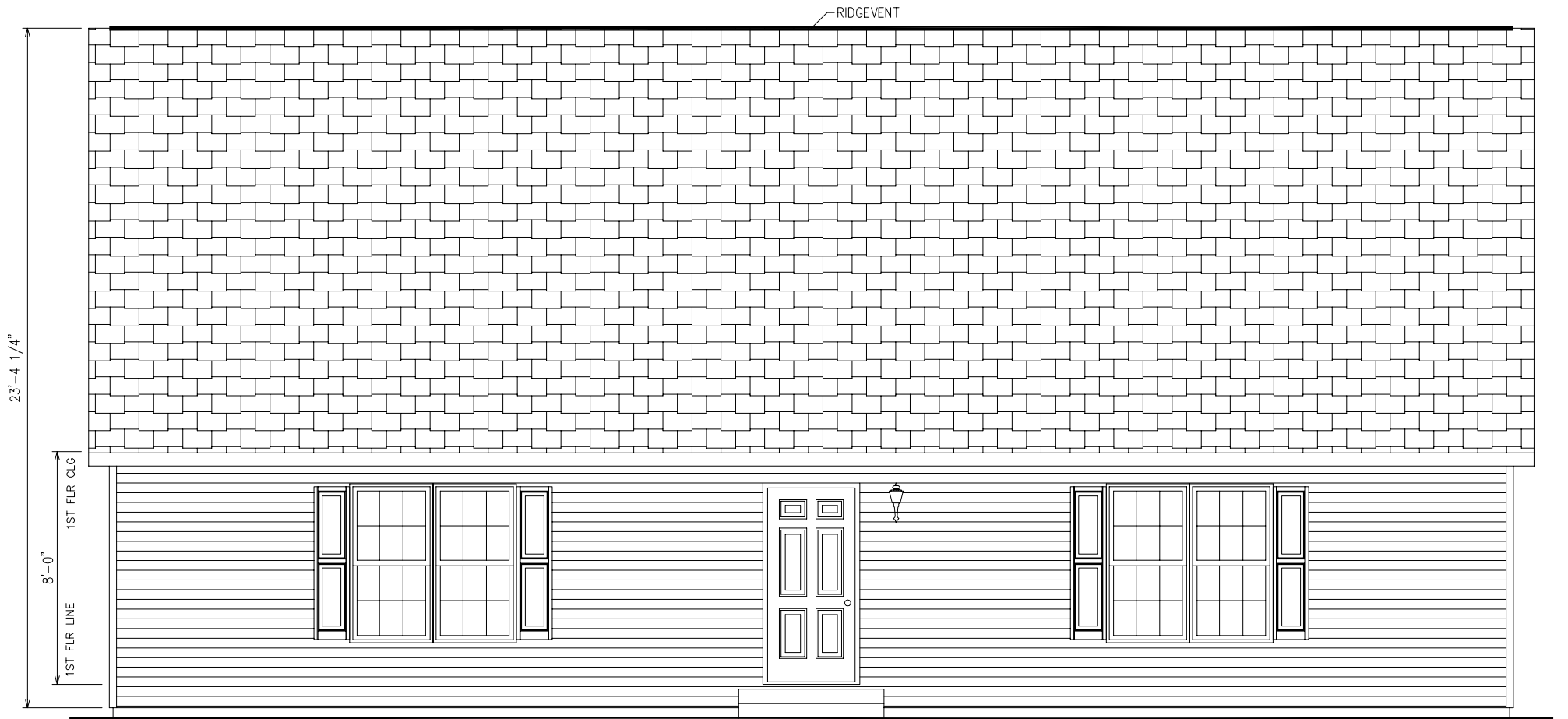
FRONT ELEVATION
