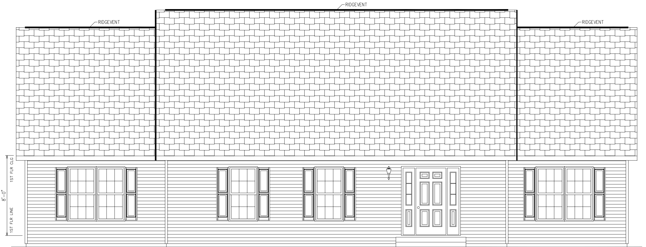
FRONT ELEVATION
