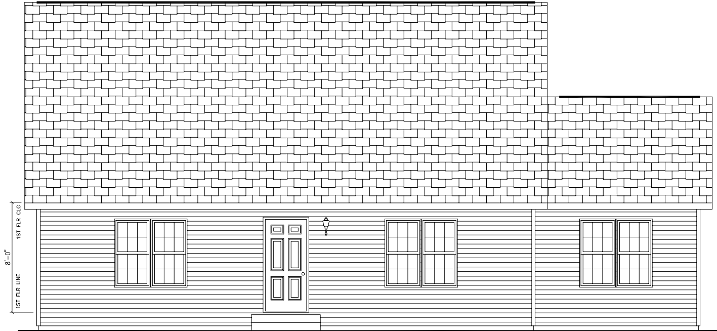
FRONT ELEVATION
