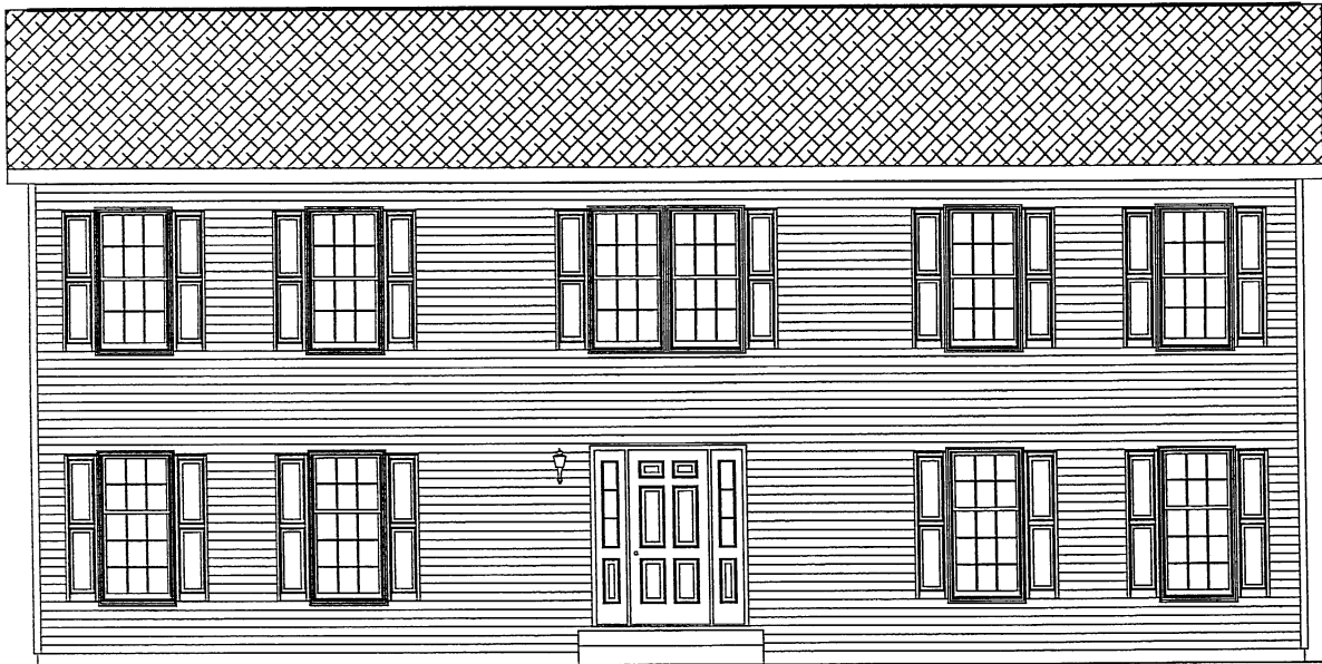
FRONT ELEVATION
