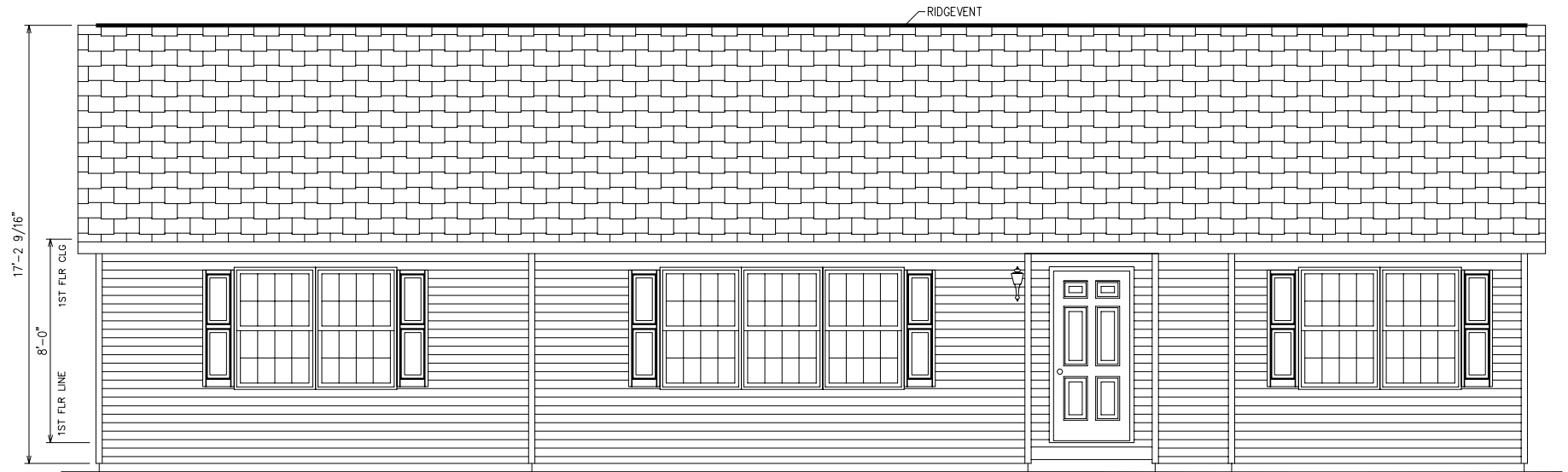
FRONT ELEVATION
