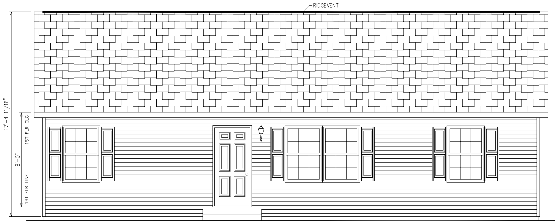
FRONT ELEVATION
