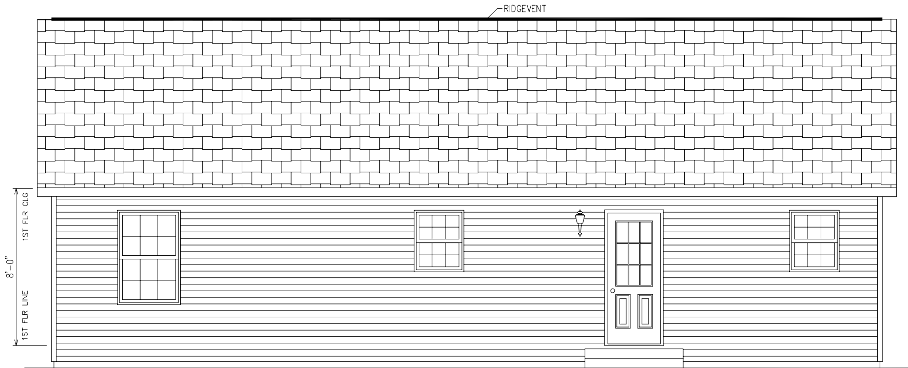
REAR ELEVATION
