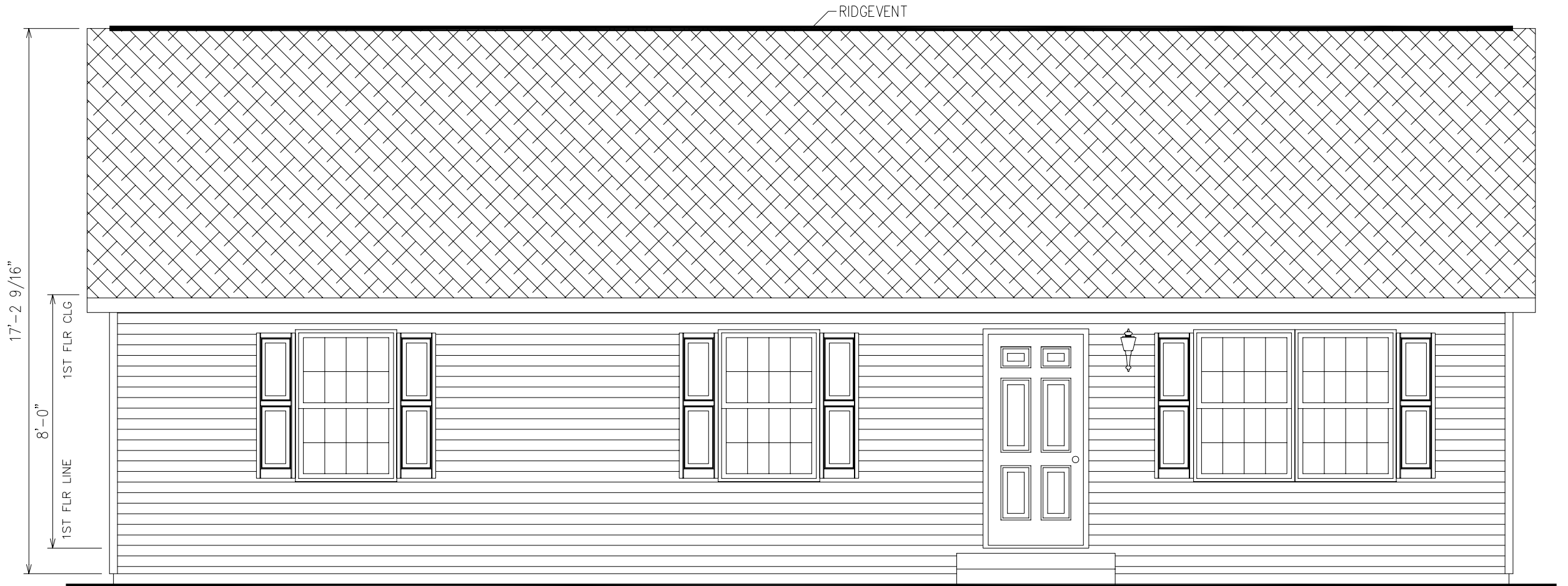
FRONT ELEVATION
