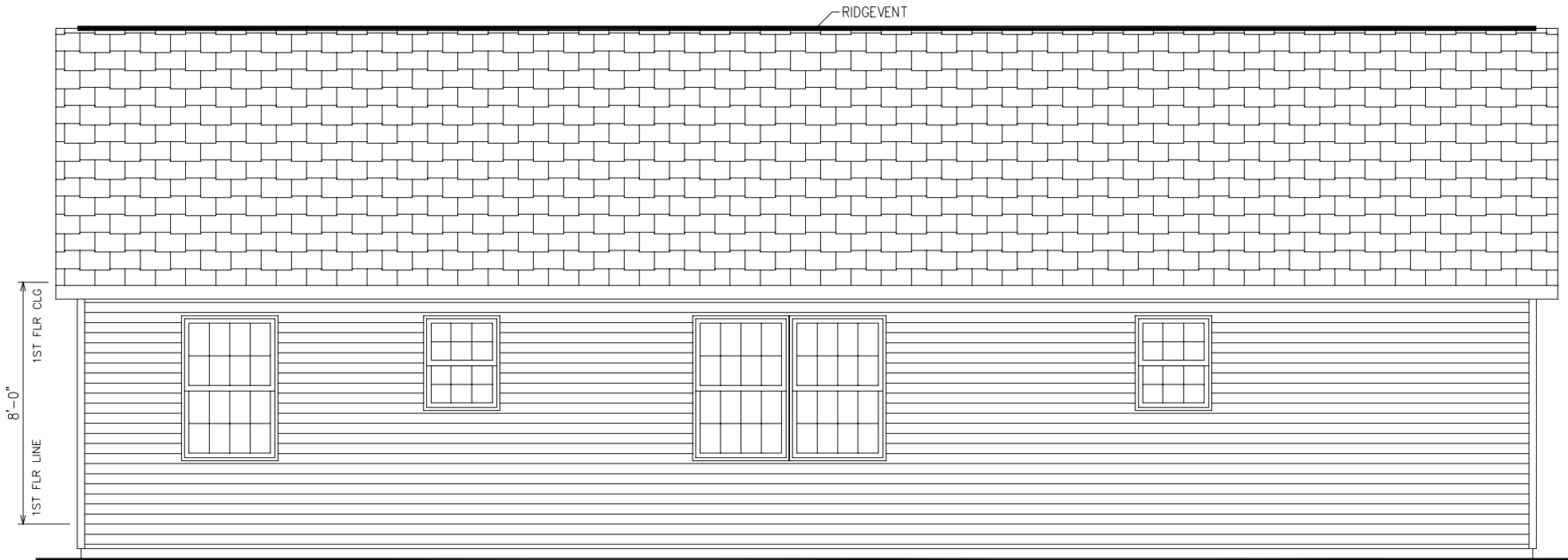
REAR ELEVATION
