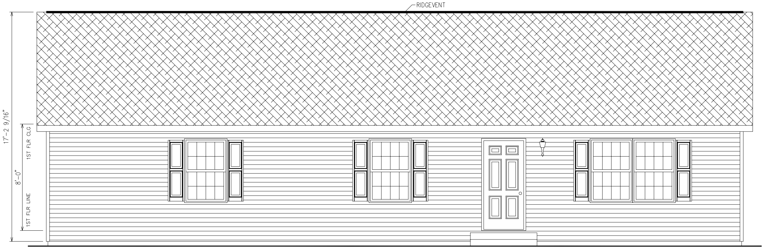
FRONT ELEVATION
