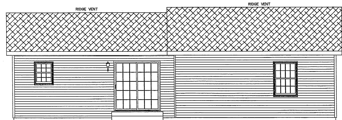
REAR ELEVATION
