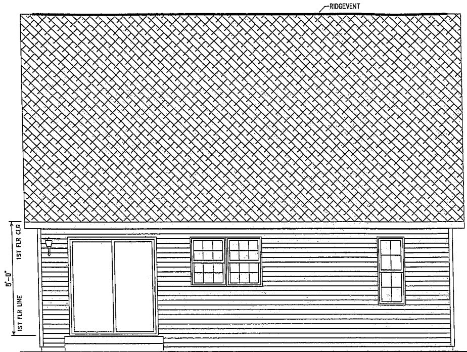
REAR ELEVATION
