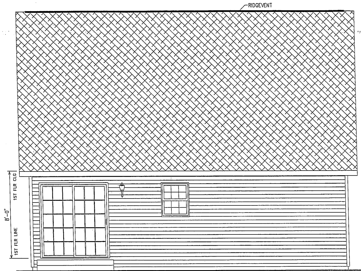
REAR ELEVATION
