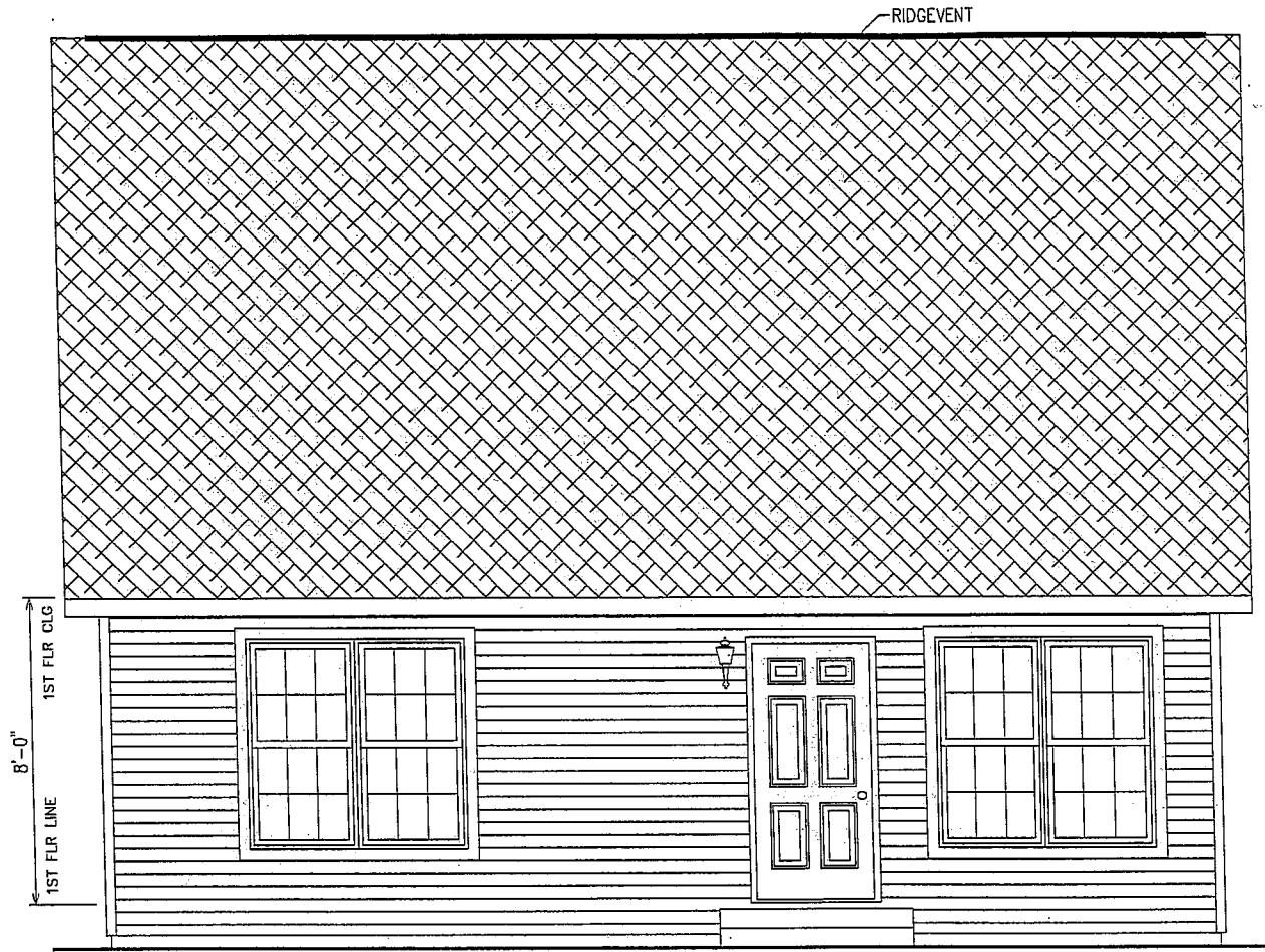
FRONT ELEVATION
