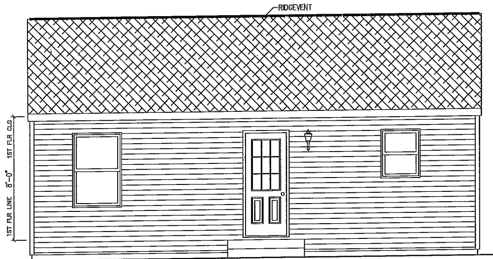
REAR ELEVATION
