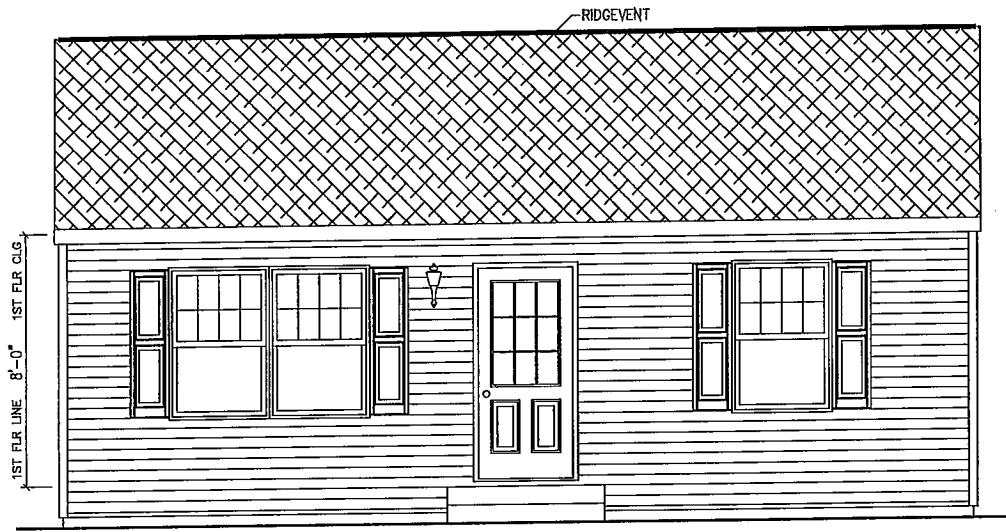
FRONT ELEVATION
