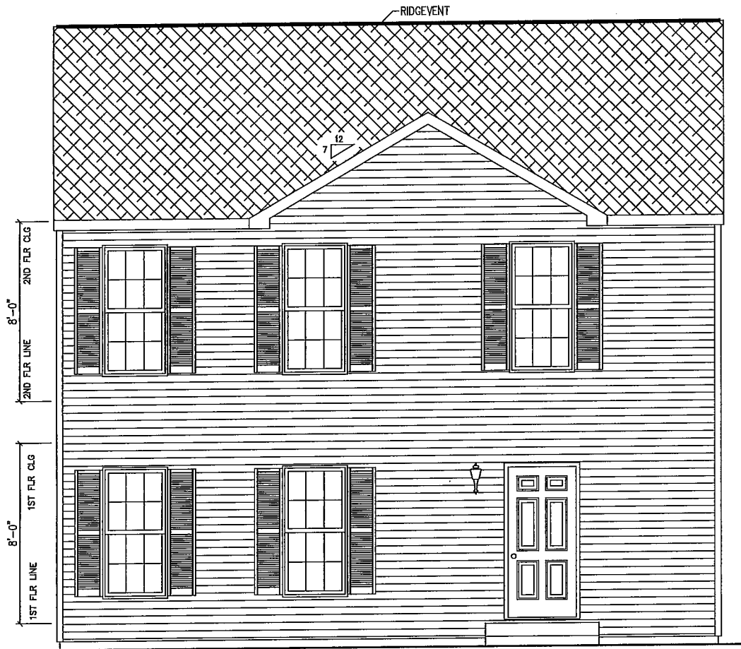
FRONT ELEVATION
