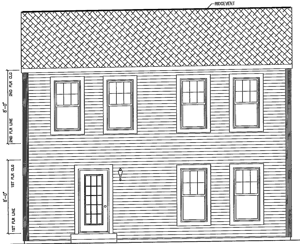
FRONT ELEVATION
