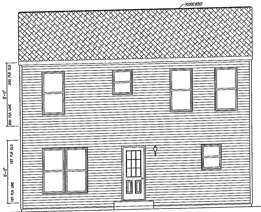
REAR ELEVATION
